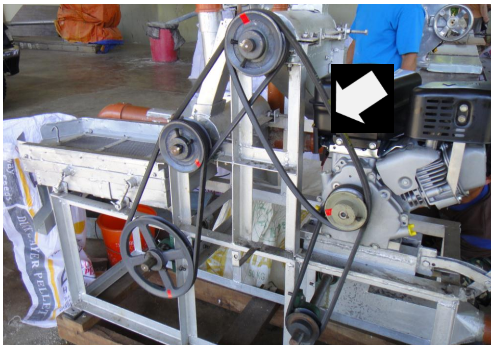
Figure 12. No belt guard
